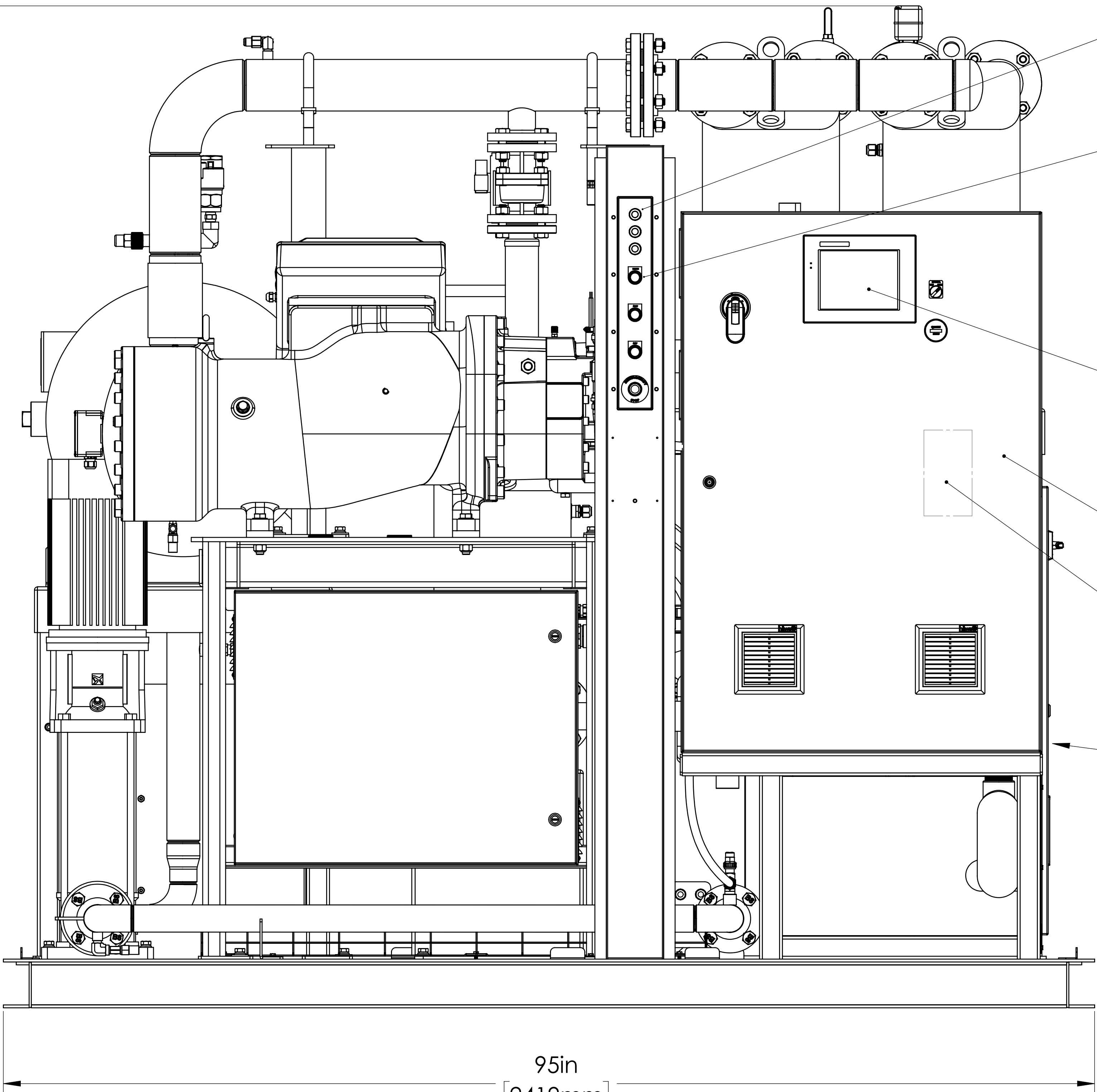
4400B SINGLE HEAT FRONT VIEW
