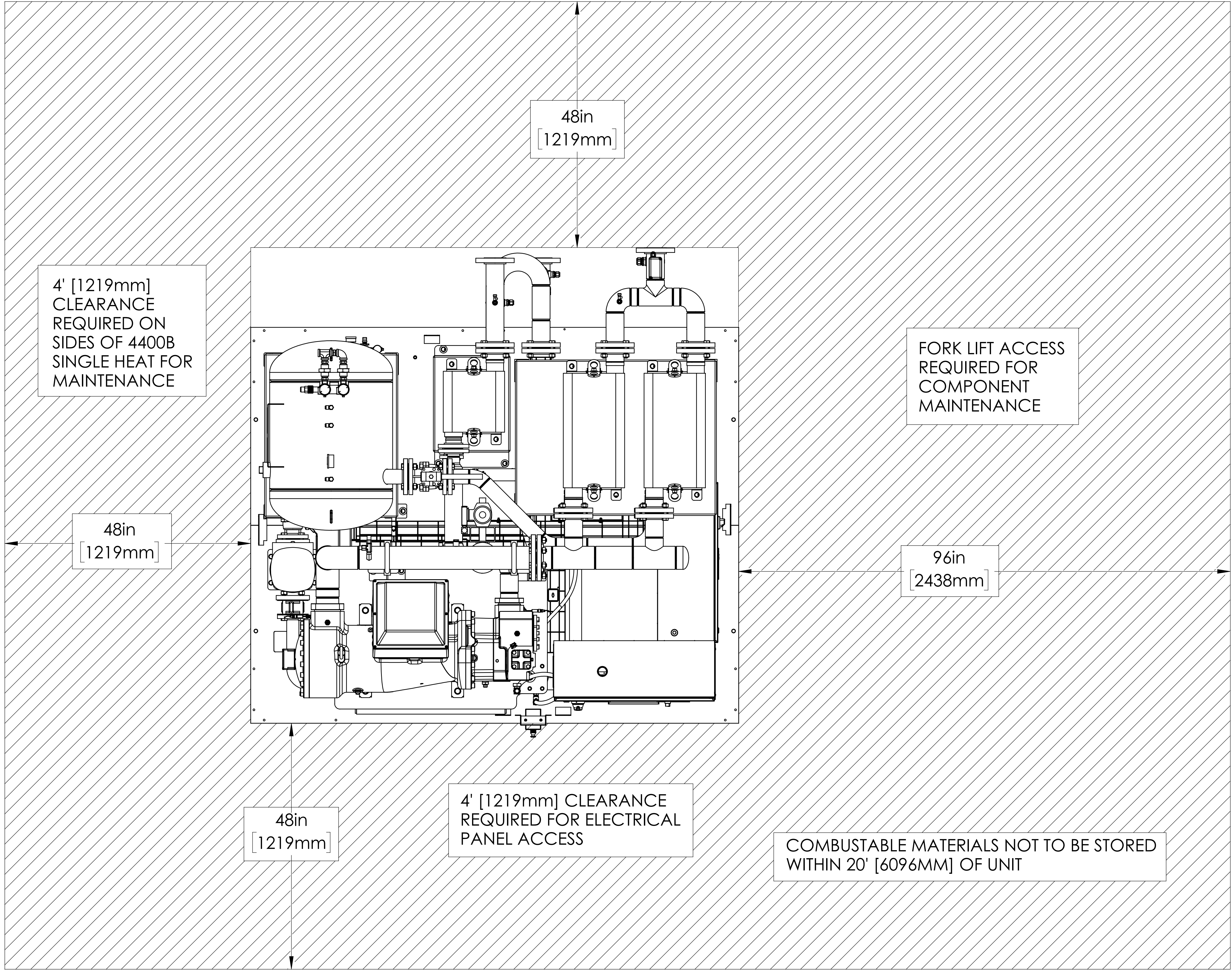
4400B SINGLE HEAT TOP VIEW
