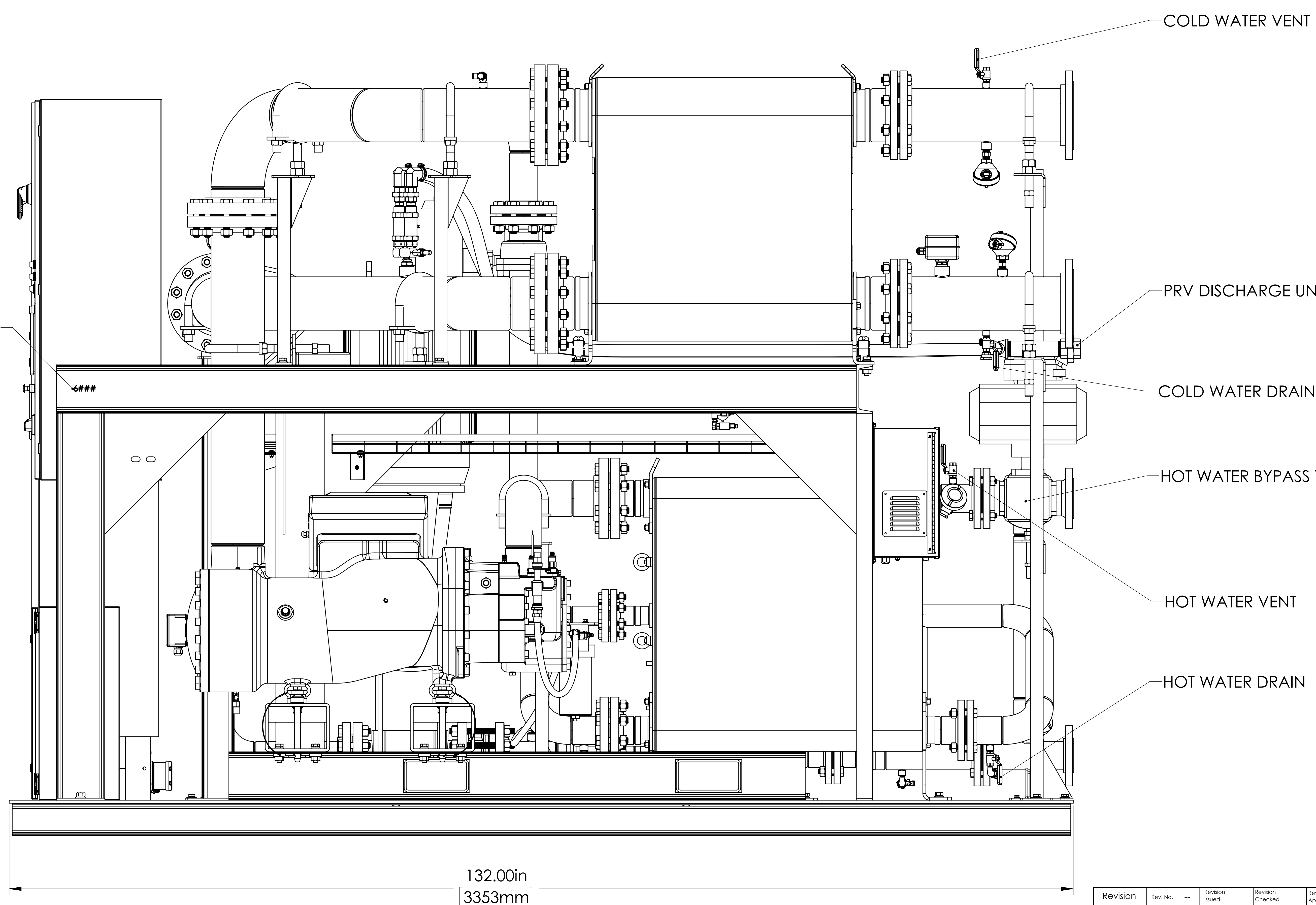
MODEL 6500B+ SINGLE HEAT SIDE VIEW
