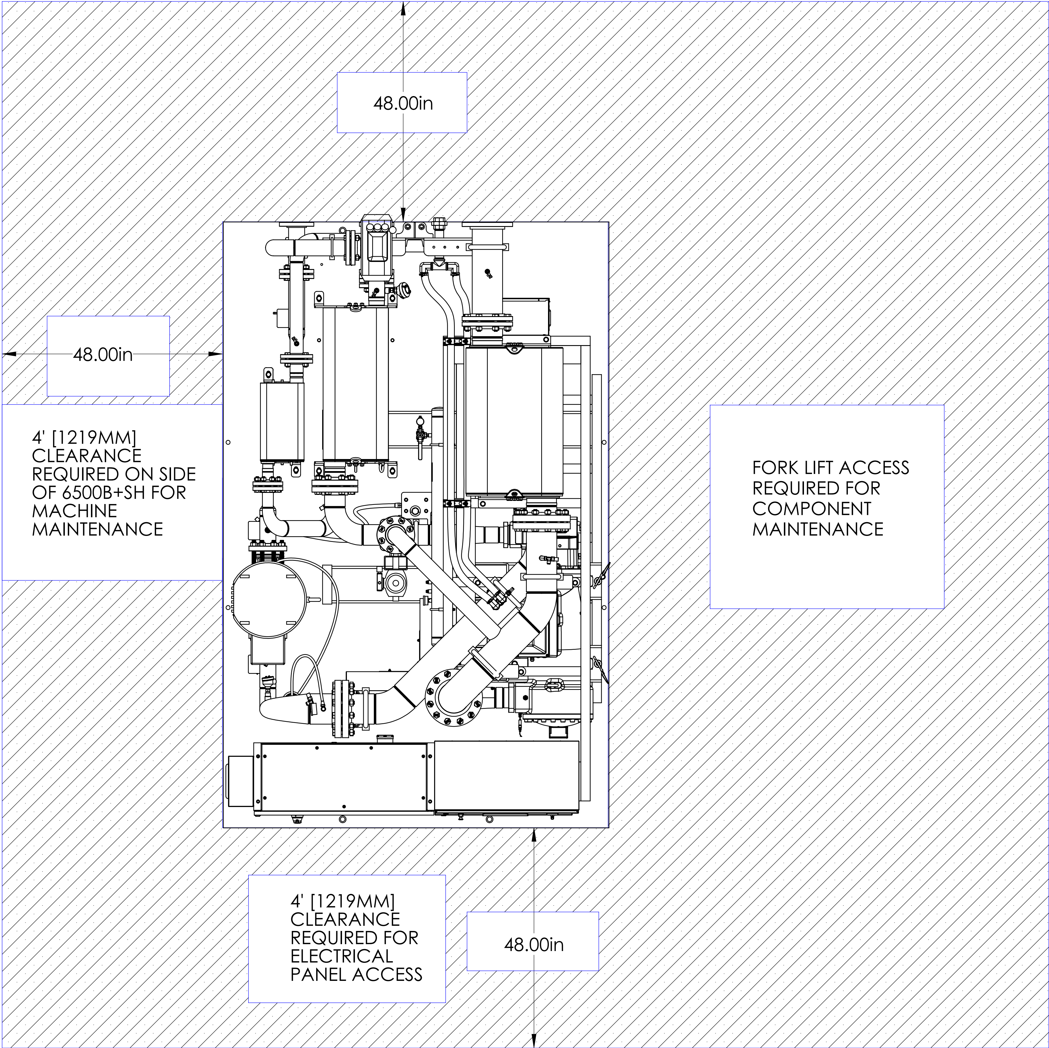
MODEL 6500B+ SINGLE HEAT TOP VIEW
