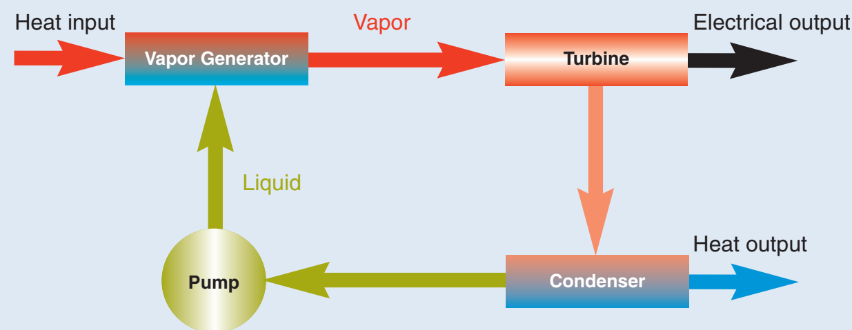
Typical ORC Configuration
